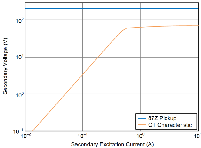
Fig. 24. Magnetization characteristic of a C50 400:5 CT and horizontal line representing the V_{87Z} = 200 V relay pickup. The horizontal line does not intersect the CT characteristic.
