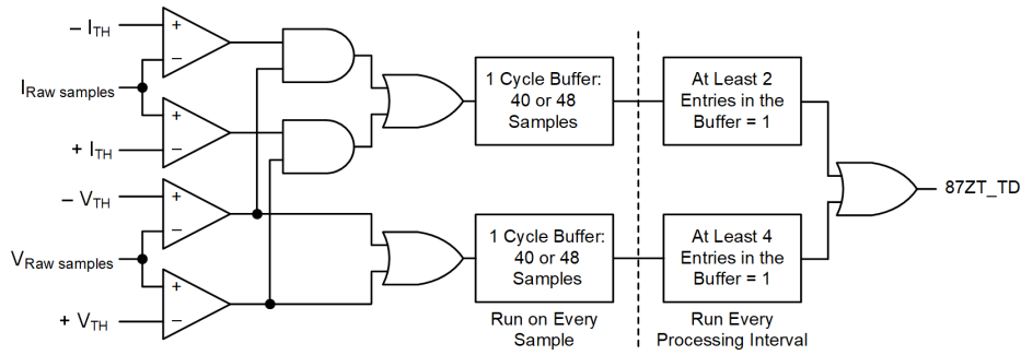
Fig. 2. Waveshape recognition element logic.
