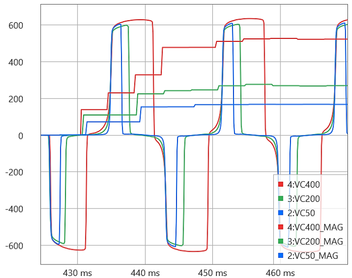
Fig. 13. The voltage magnitudes estimated by the relay digital filter are directly affected by the CT accuracy class voltage.
