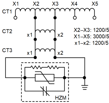
Fig. 18. Mismatched CT connection that uses the matching tap of the higher ratio CT.
