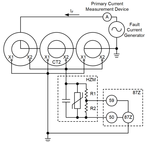
Fig. 5. Setup for testing the 87Z relay.
