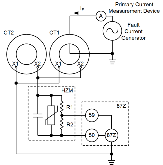
Fig. 23. Test setup to experimentally determine the magnetizing current of the CTs at the 87Z setpoint voltage.
