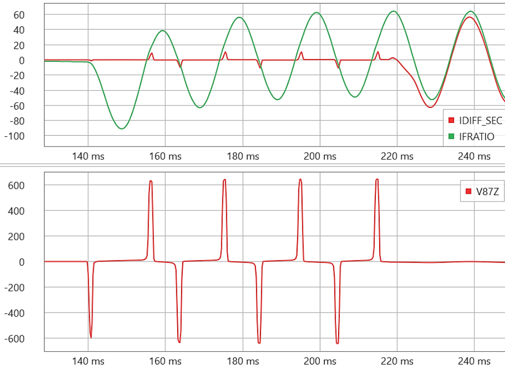
Fig. 7. Differential and ratio currents (top) and stabilizing resistor voltage (bottom) recorded by the 87Z relay during an internal fault test.
