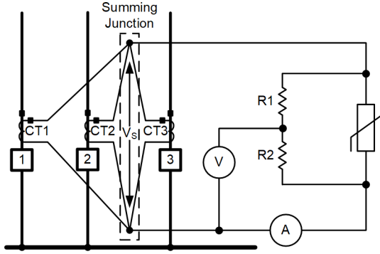
Fig. 6. Setup for testing an 87Z scheme for a range of stabilizing resistance values, CT classes and ratios, and MOV maximum clamping voltages.
